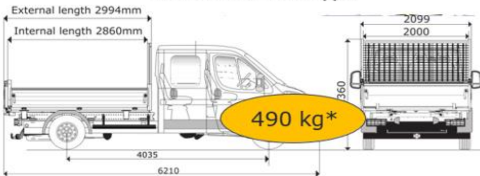
L3 Chassis Crew Cab (7 seats) : 2900 tipper
